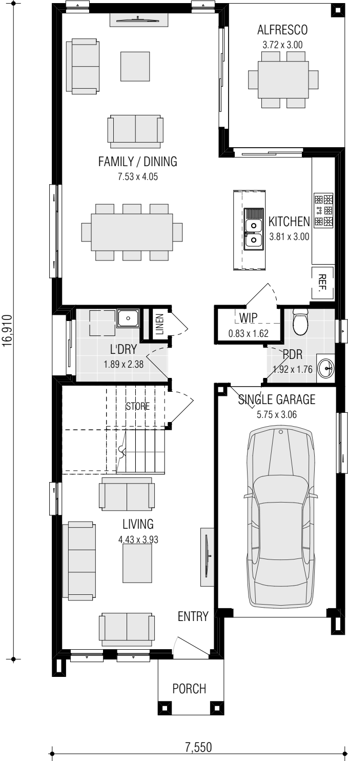
GROUND FLOOR
