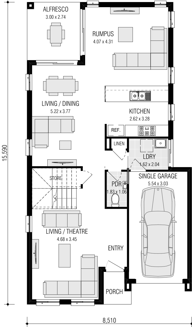
GROUND FLOOR
