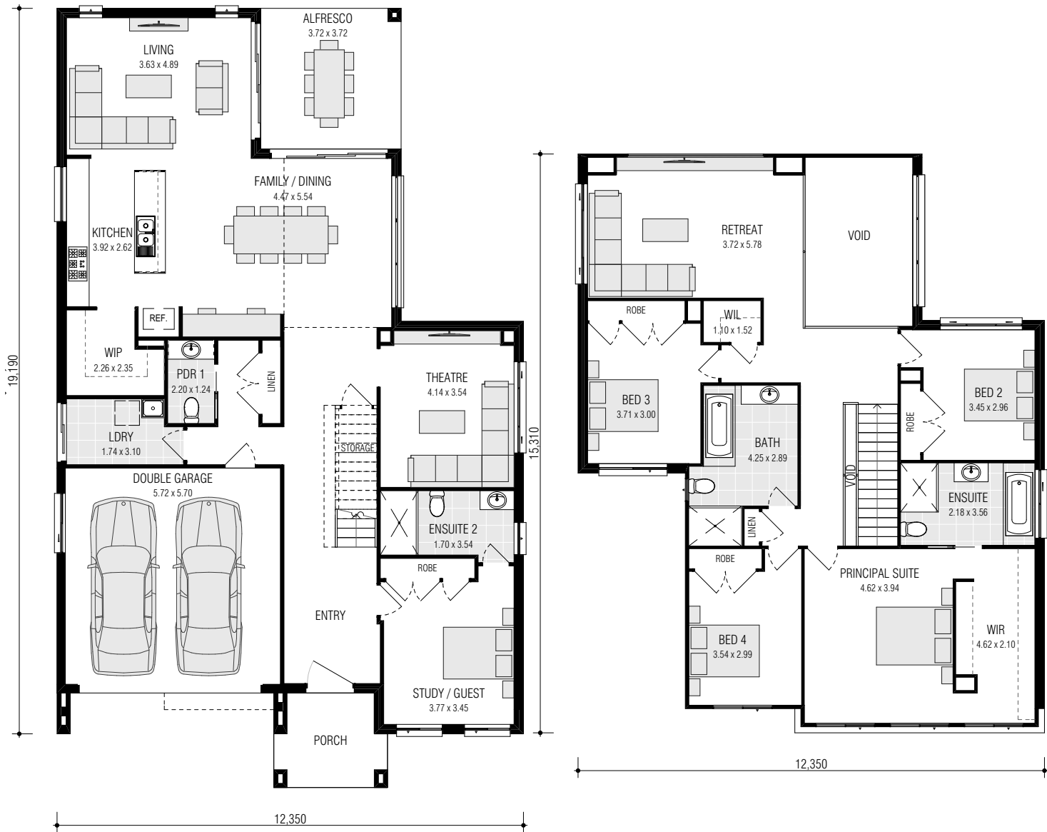
Ground Floor
