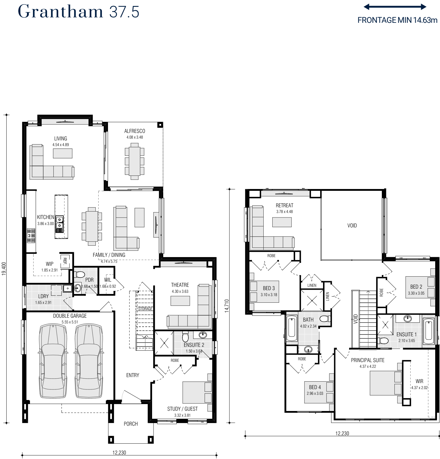
Ground Floor
