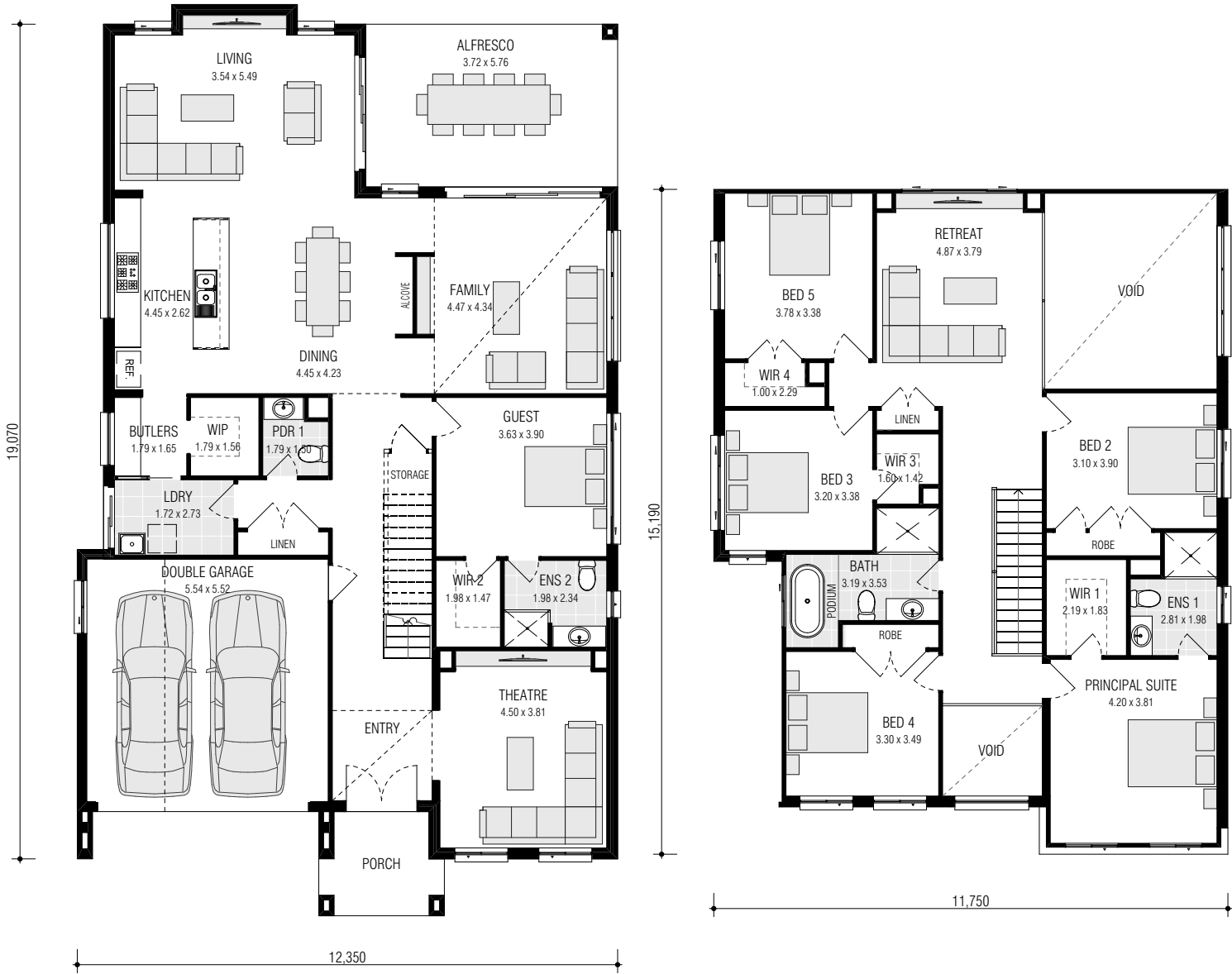
Ground Floor
