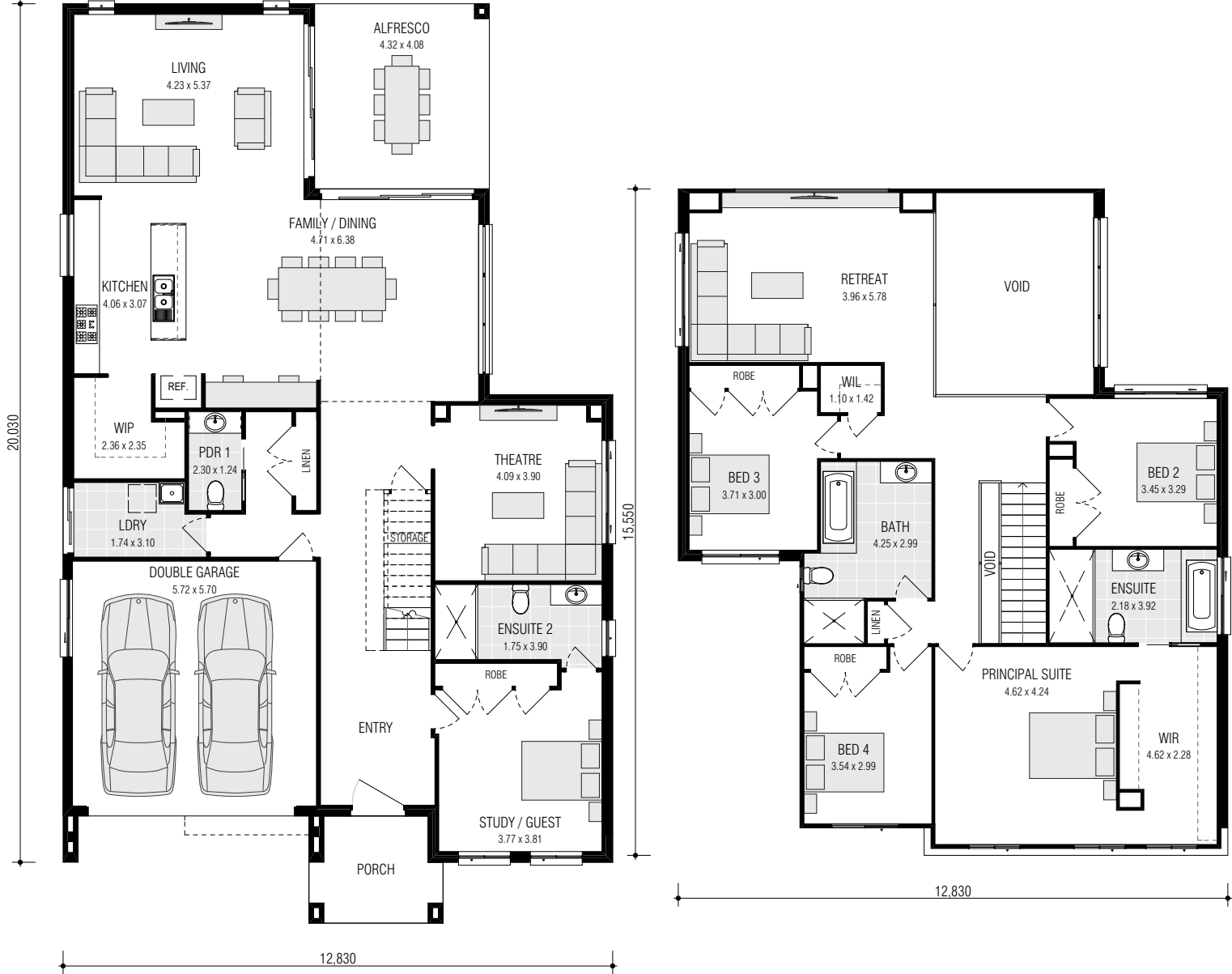
Ground Floor
