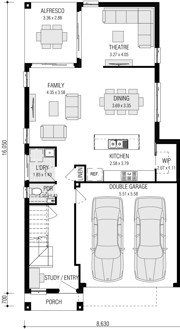
GROUND FLOOR
