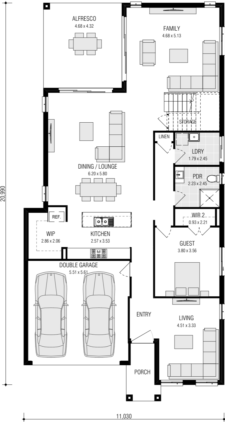
Ground Floor
