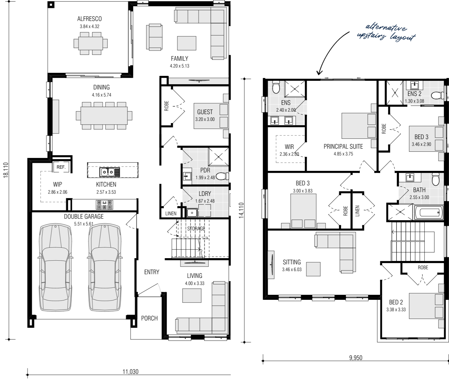
Ground Floor
