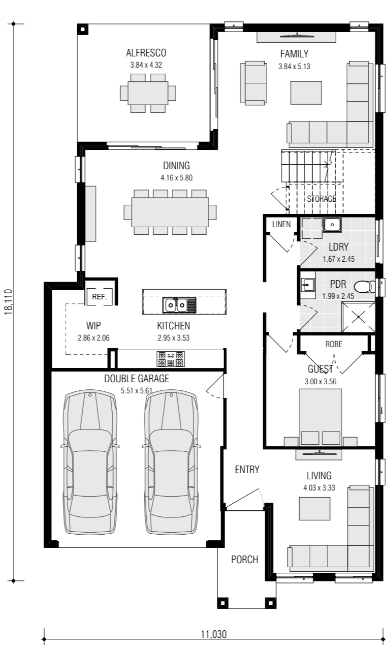
Ground Floor
