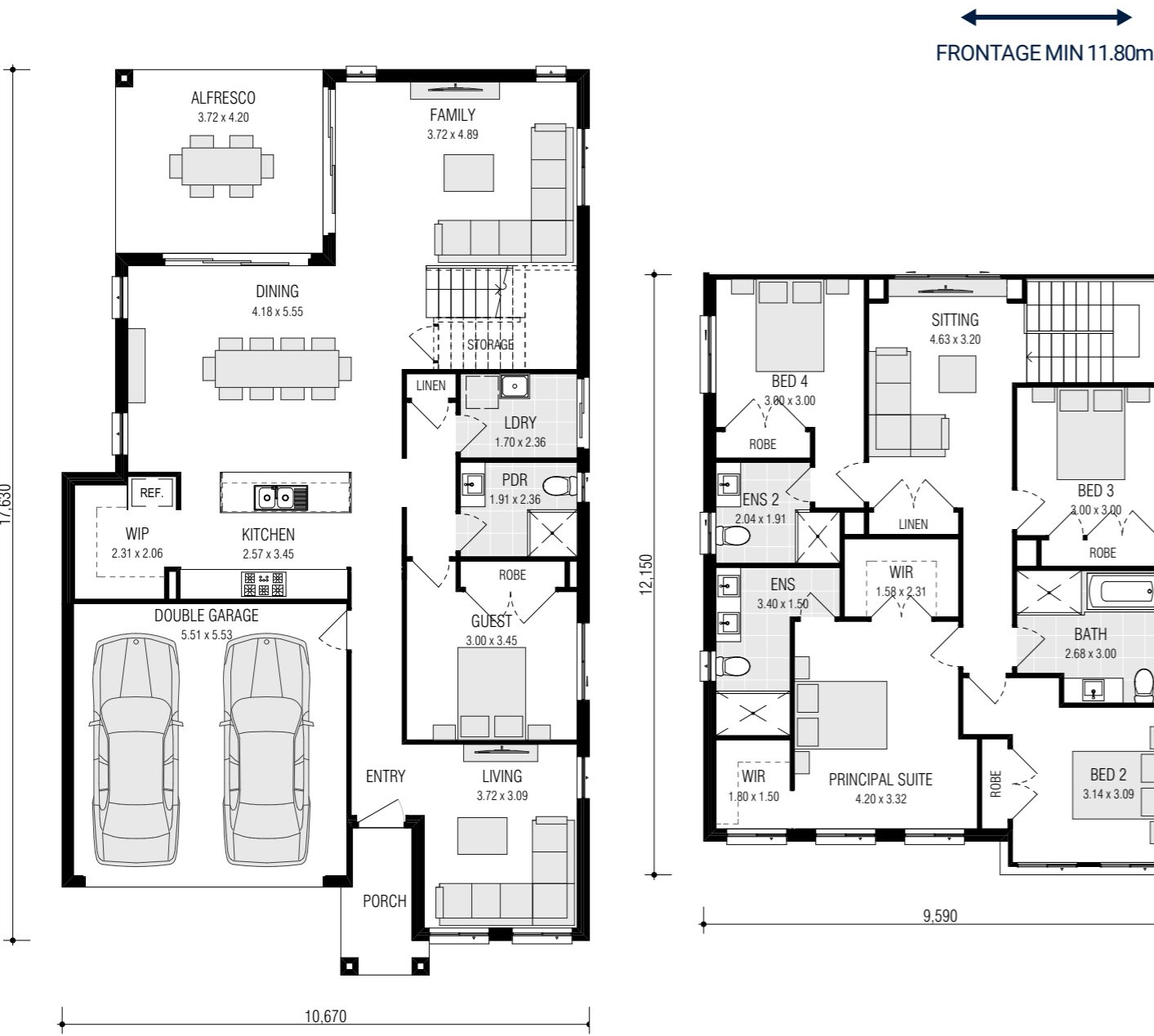
Ground Floor
