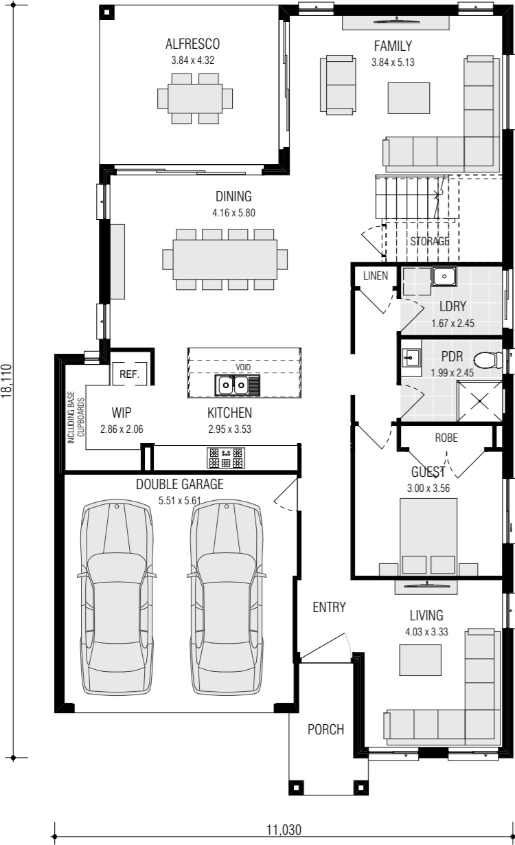
Ground Floor
