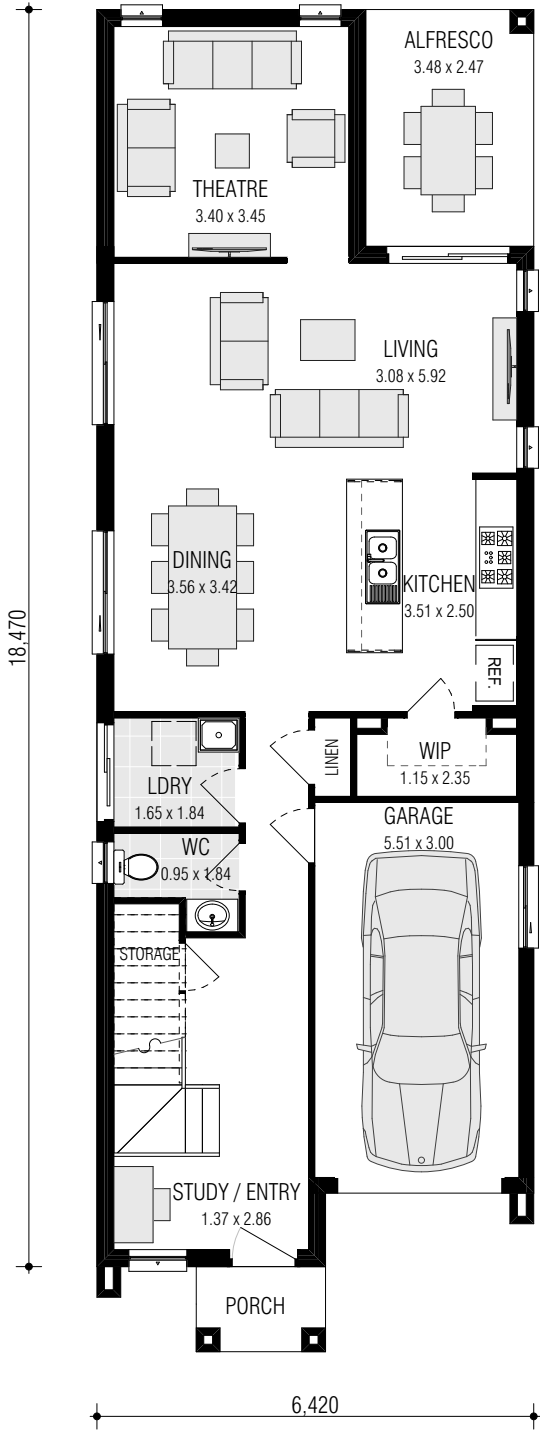
Ground Floor
